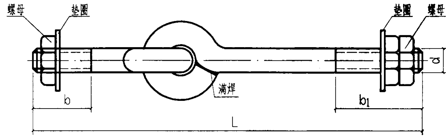
环眼双头螺纹吊杆
