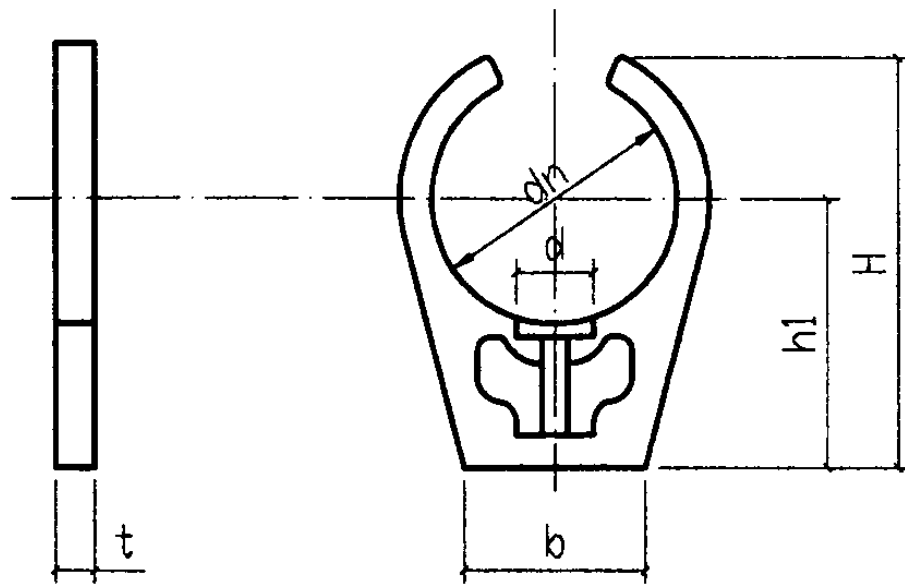
开口式管夹
