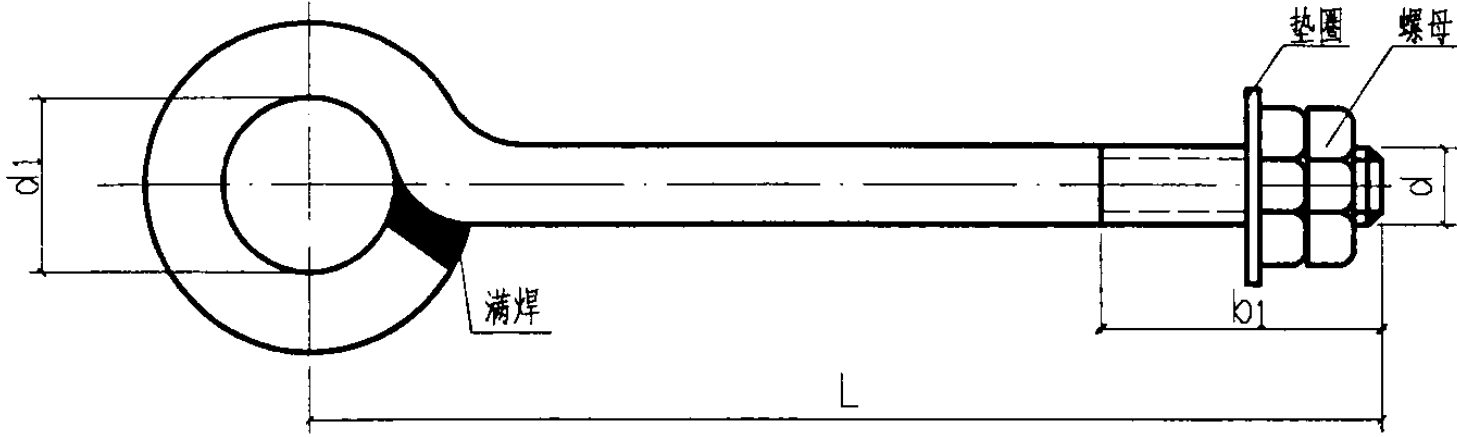
闭口环眼单头螺纹吊杆
