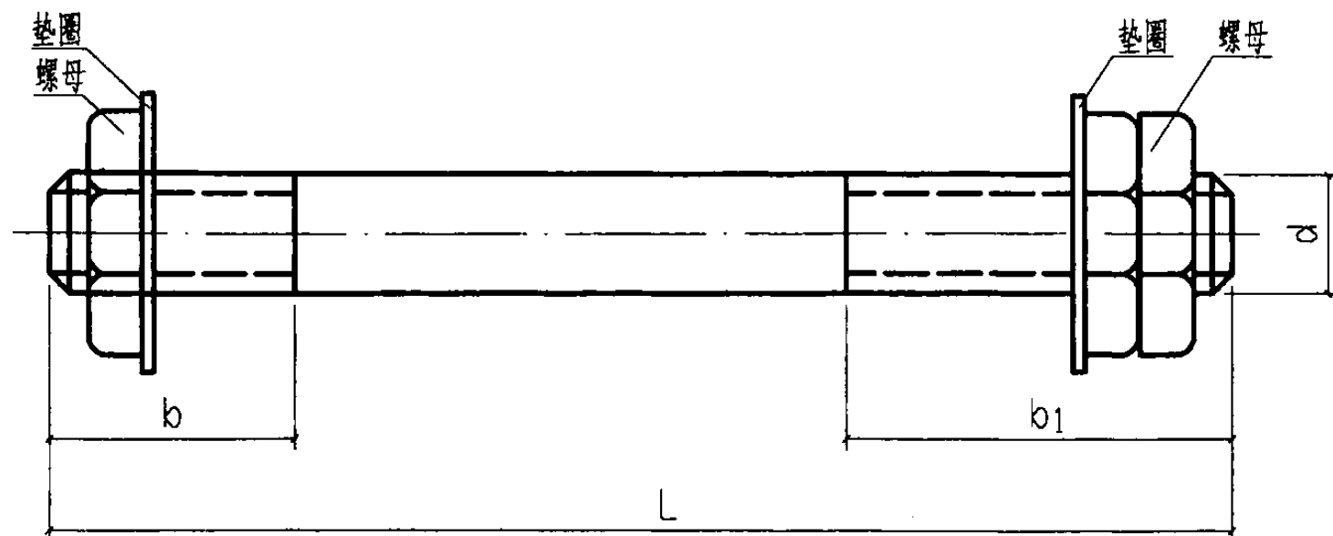
双头螺纹吊杆
